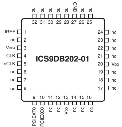
32-Lead VFQFN 5mm x 5mm x 0.95 package body K Package Top View
